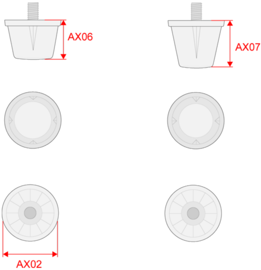
Dimensions (cm)
