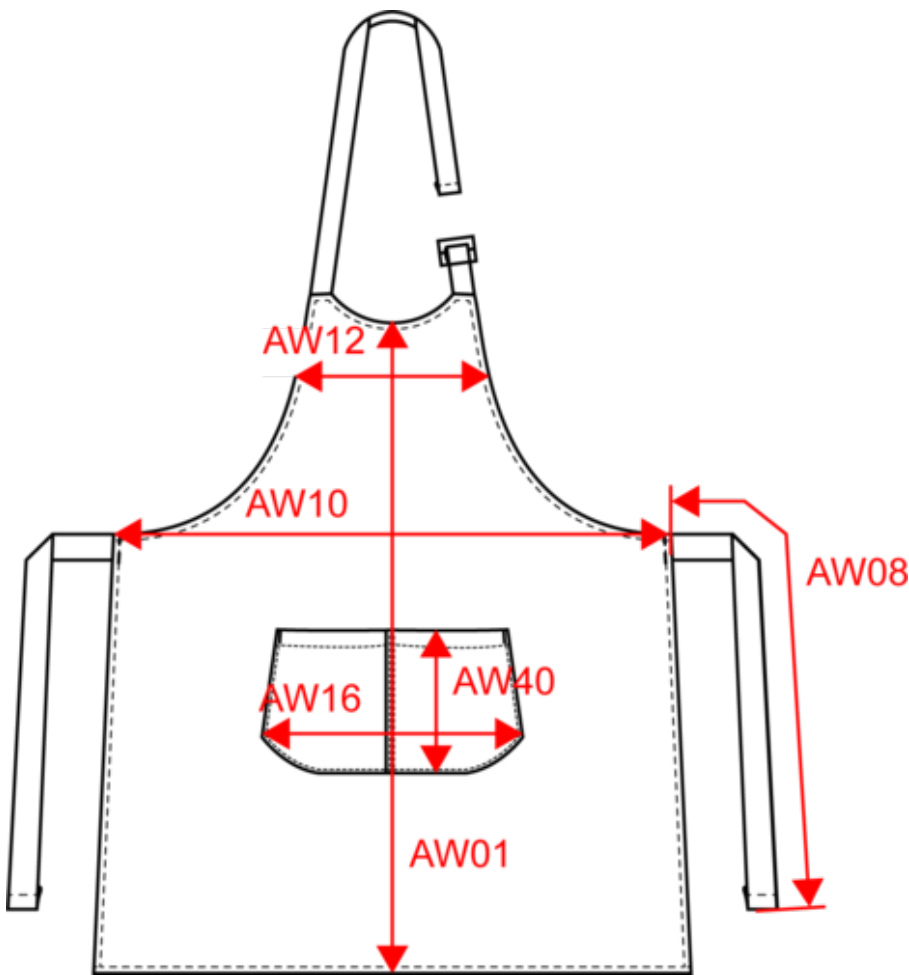
Dimensions (cm)
