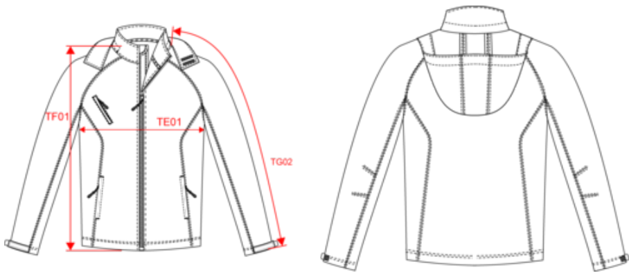
Dimensions (cm)
