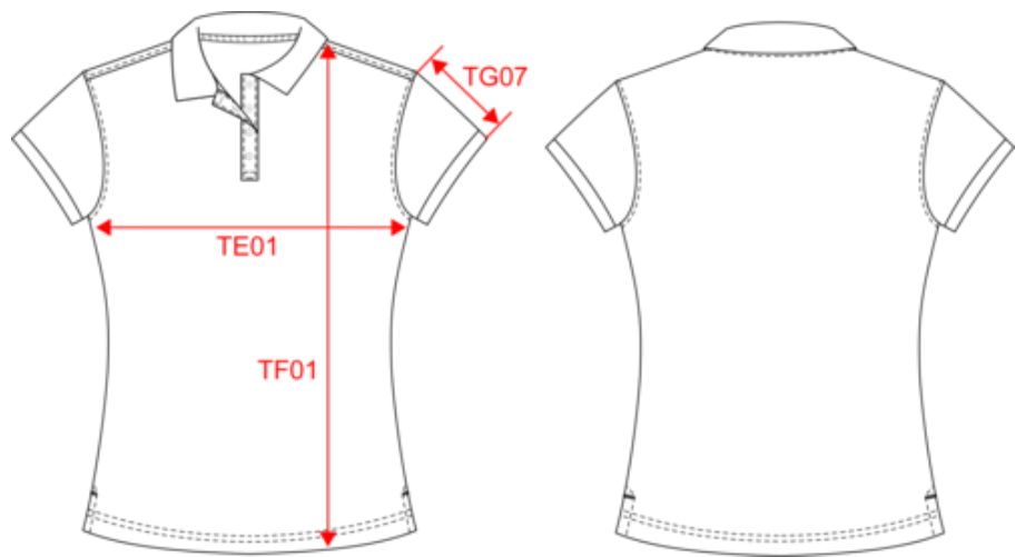
Dimensions (cm)
